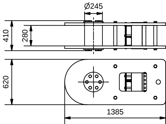
Anchor (1:30)
