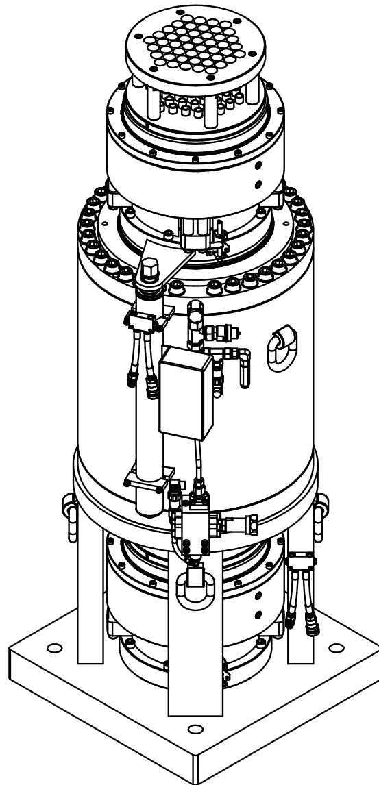
Anchor (1:30)
